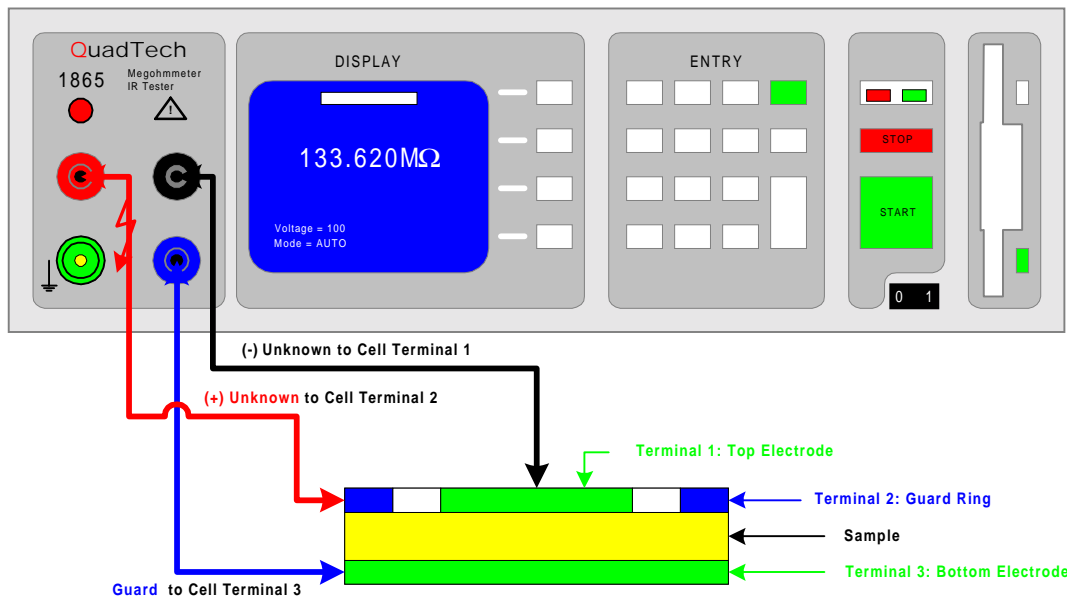
Figure 2: Connection of 1865 Megohmmeter for Surface Resistivity Measurement
