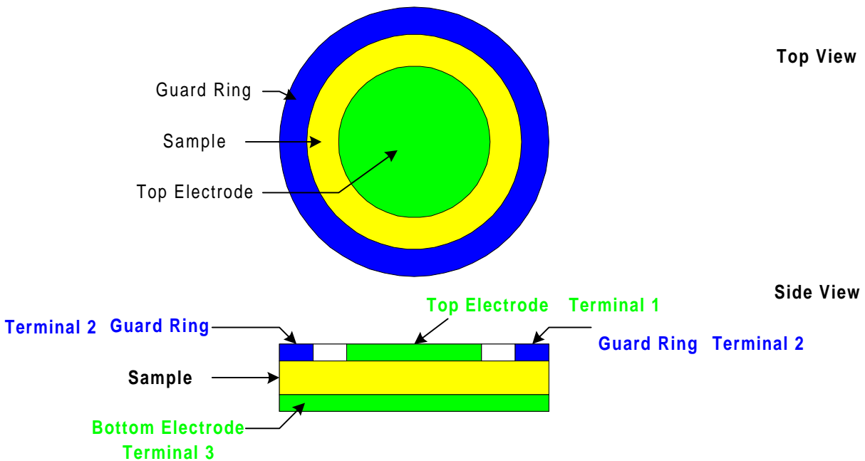
Figure 1: ASTM D257 Test Cell
